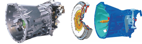
Mercedes Benz Licensed G-32, 5 Speed Gear Box with dual mass fly wheel
